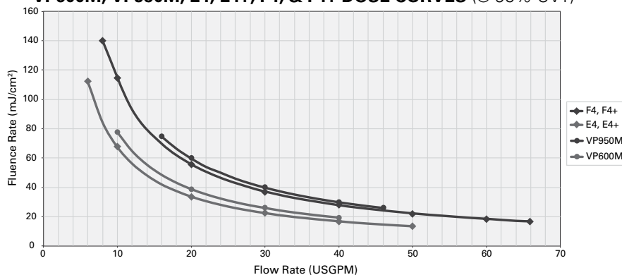
VP600M, VP950M, E4, E4+, F4, & F4+ DOSE CURVES (@ 95% UVT)
